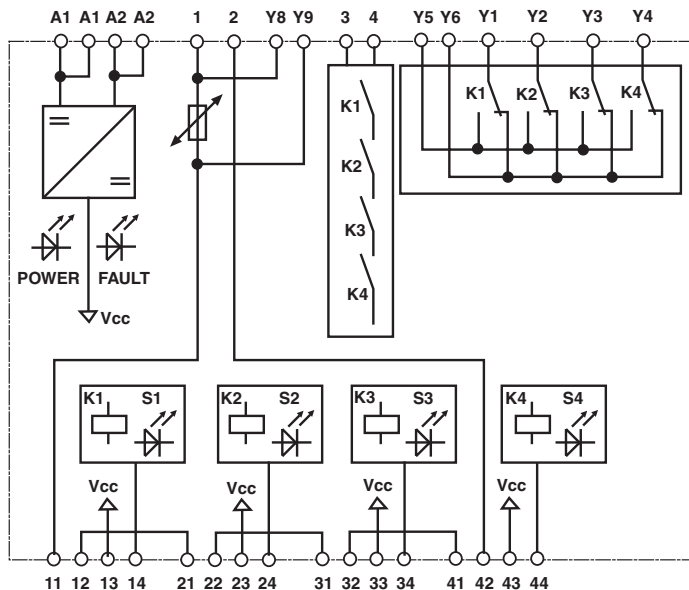
Internal wiring diagram
